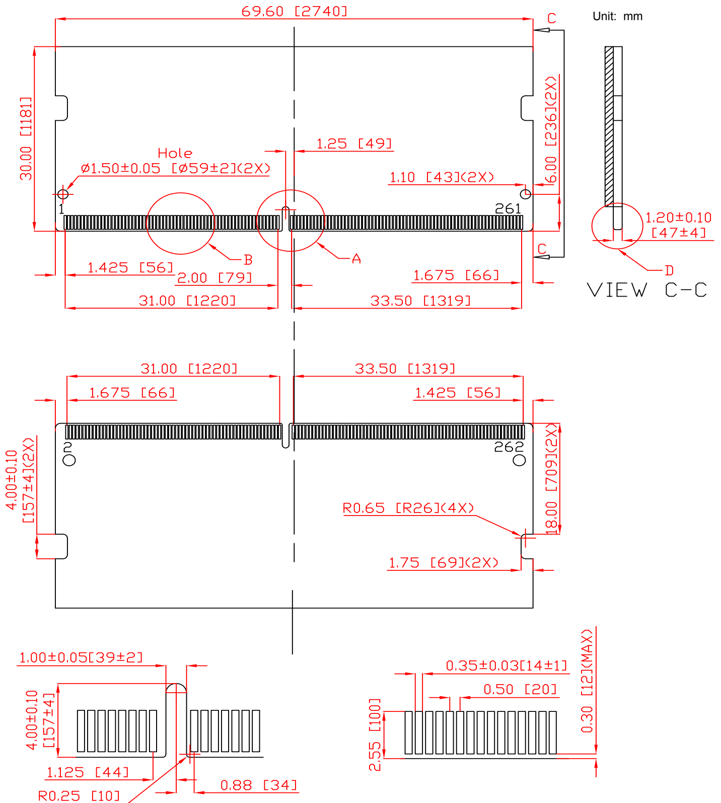
Detail A
