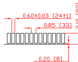
Detail B
